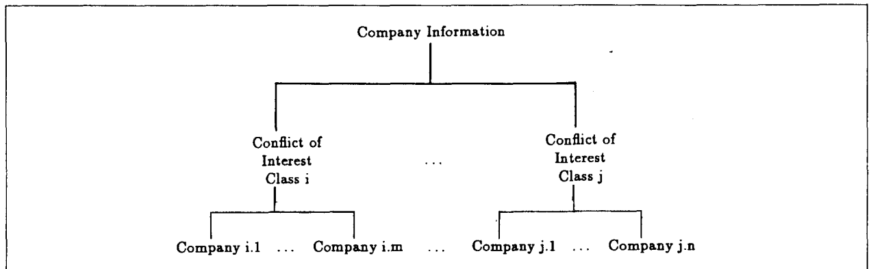
Fig. 1. Company information in the Chinese Wall policy.
