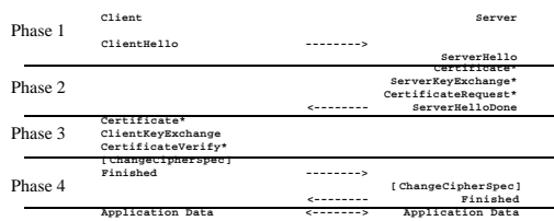
Fig. 1 - Message flow for a full handshake * Indicates optional or situation-dependent messages that are not always sent.
