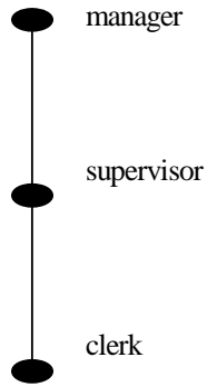
Figure 2. Role Hierarchy
